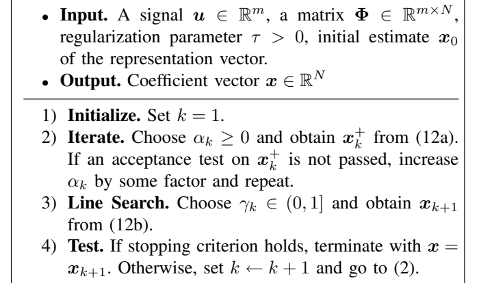
Fig. 3. Gradient Descent Framework
