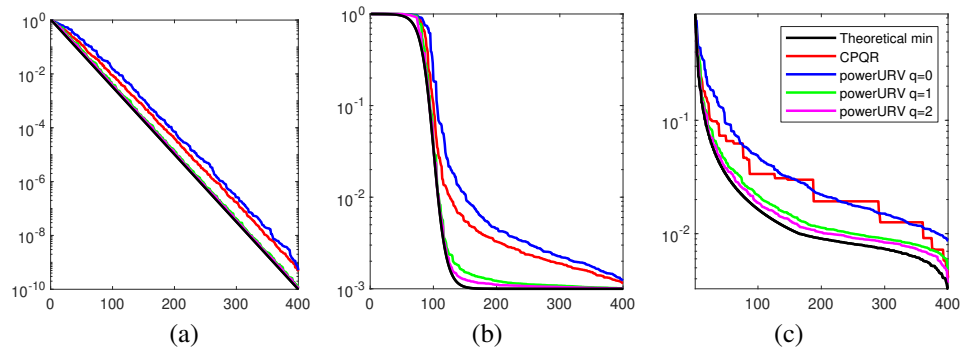
FIGURE 2. The rank-revealing ability of CPQR and powerURV for different values of the power parameter q , as discussed in Section 16.3. The error e_k = \|\mathbf{A} - \mathbf{U}(:, 1 : k)\mathbf{R}(1 : k, :)\mathbf{V}^*\| (see (16.2)), is plotted versus k for three different matrices \mathbf{A} of size 400 \times 400 . The black lines plot the theoretical minimal values \sigma_{k+1} . (a) A matrix whose singular values decay rapidly; we see that all methods perform well. (b) A matrix whose singular values plateau; we see that CPQR performs poorly, and so does the randomized method unless powering is used. (c) A discretized boundary integral operator whose singular values decay slowly; we again see the high precision of powerURV for q = 1 and q = 2 .
